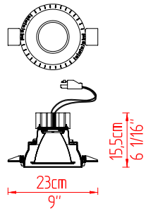
F19 F54 01 LED
