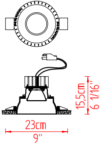
F19 F53 01 LED
